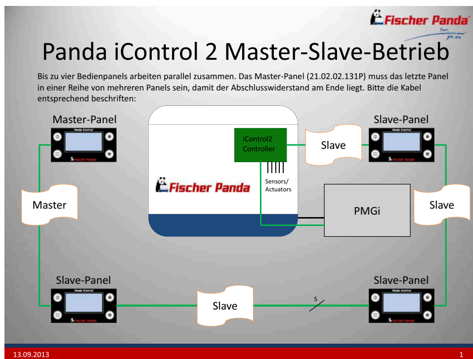
Fig. 16.5-1: Master Slave Schema
