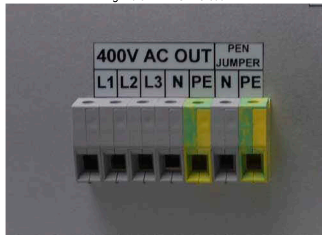
Fig. 20.5-3: PMGi AC out
