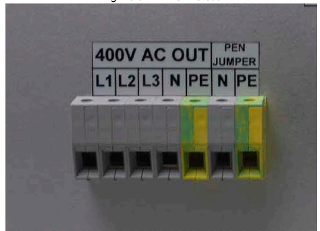
Fig. 13.5-3: PMGi AC out
