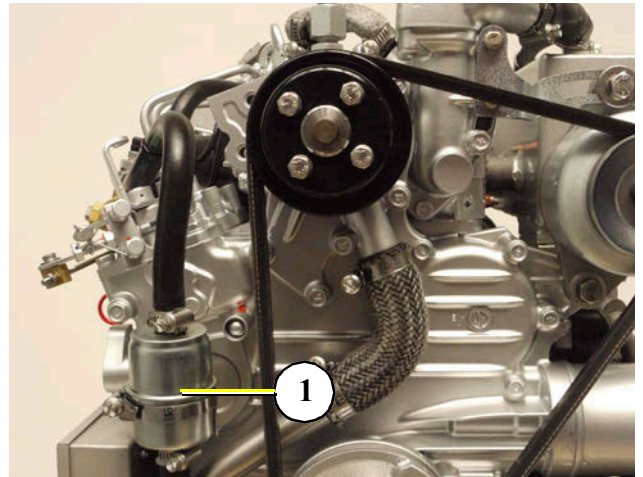
Fig. 11.4.2-1: Fuel filter
