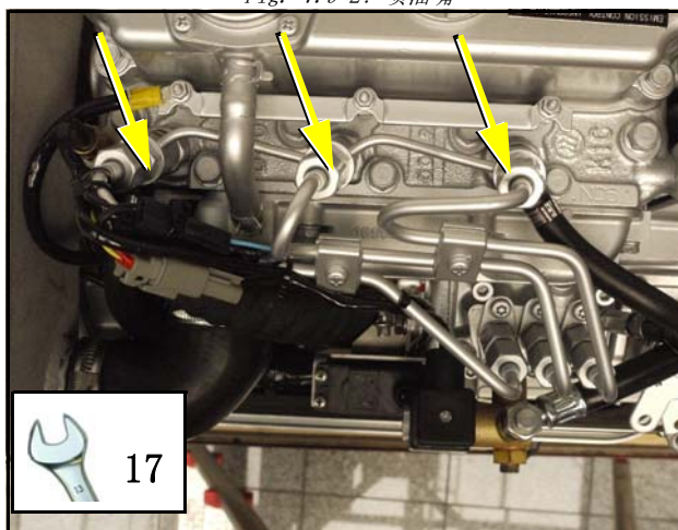
Fig. 7.9-2: 喷油嘴
